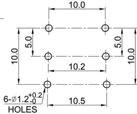
P.W.B MOUNTING DETAIL
